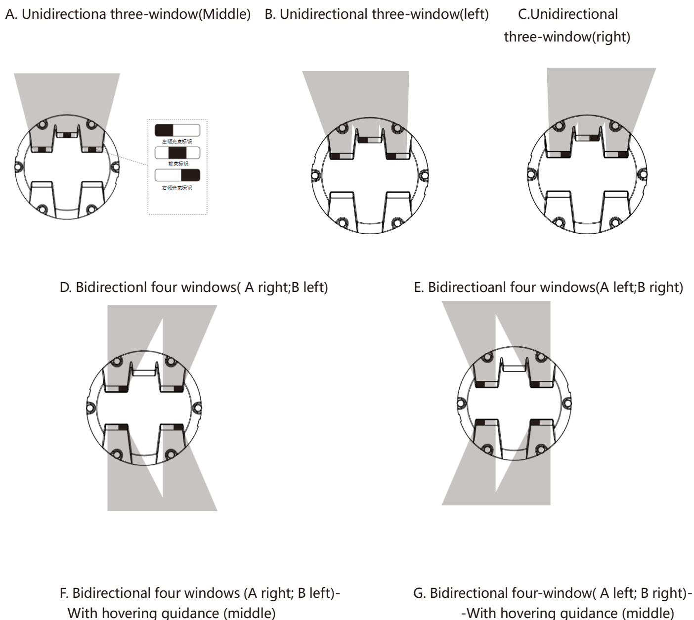
Figure 5 – 12-inch inset light fixture light emitting direction identification
