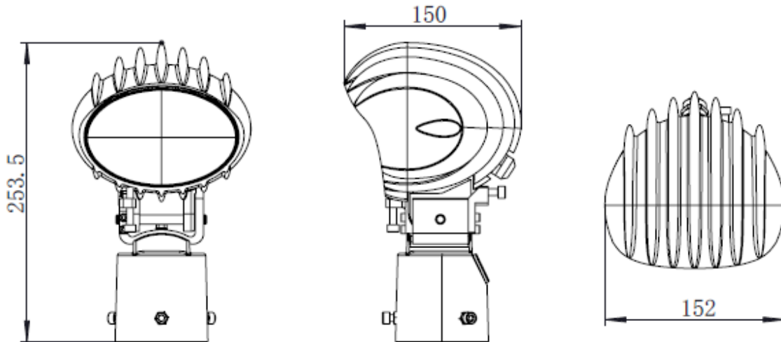
Figure 2 – Major Dimensions of the Light Fixture
