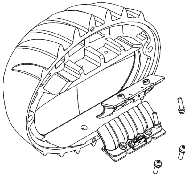
Figure 11 – Assembly and Disassembly of the Optical Components
