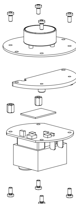
Figure 8 Installation and Removal driver module to/from optical components
